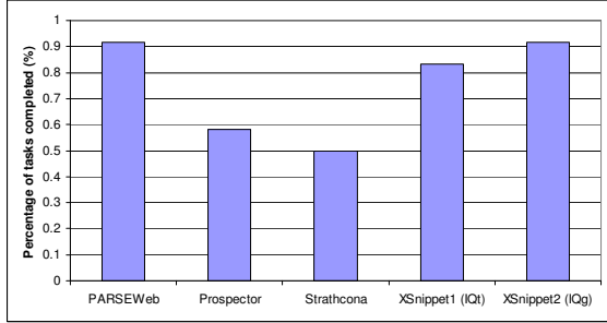
Figure 2. Evaluation results of PARSEWeb with related tools Prospector, Strathcona, and XSnippet
